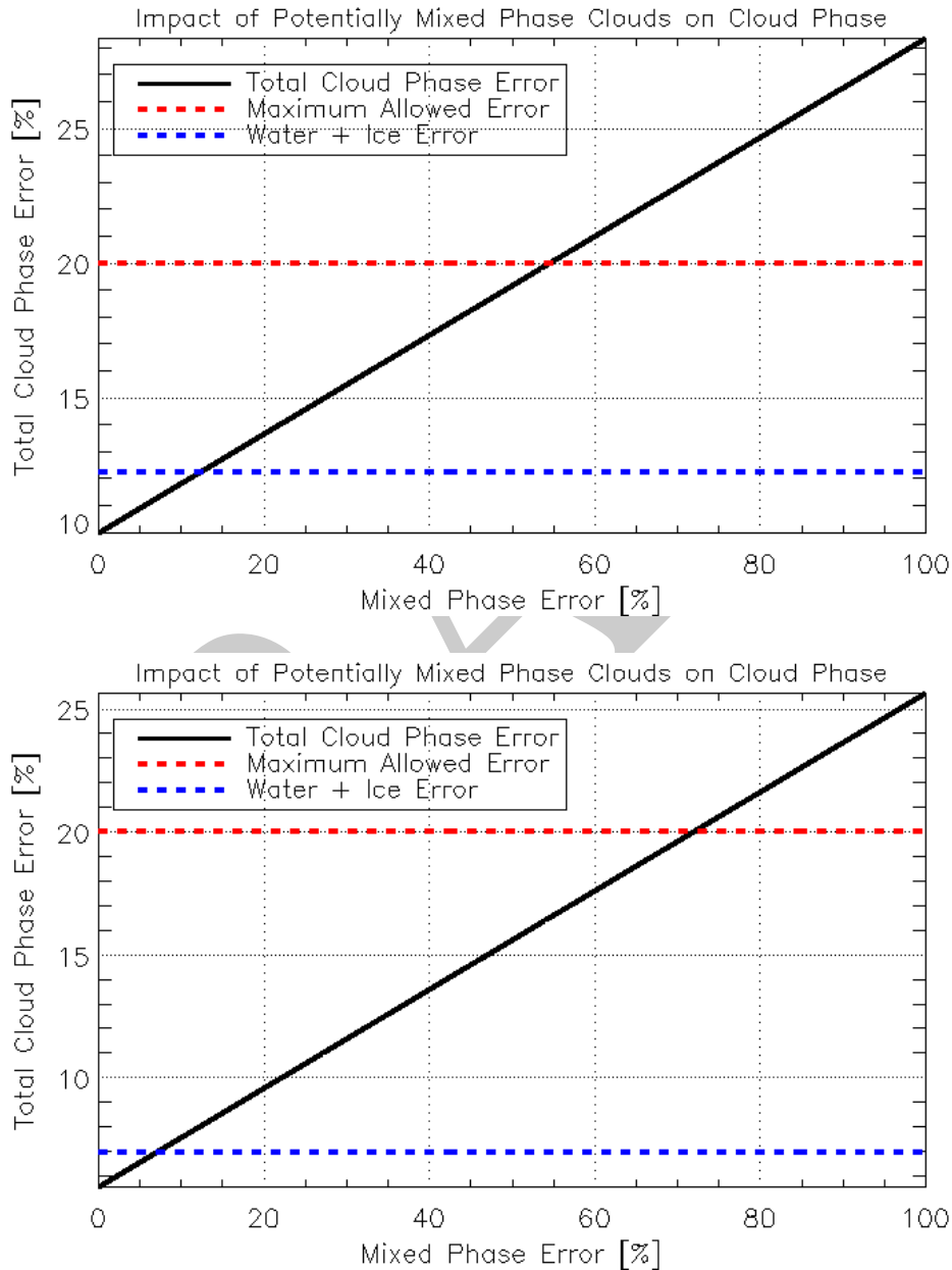
Figure 19: The total cloud phase error as a function of the assumed error in classifying potentially mixed phase clouds is shown when the minimum cloud optical depth qualifier is ignored (top) and when it is applied (bottom) with the solid black line. The dashed red line is the allowed error from the F&PS. The dashed blue line
