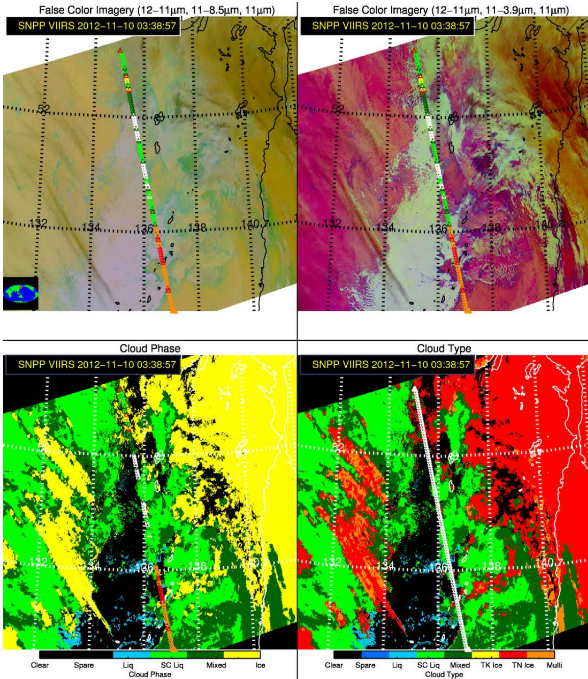
Figure 18: Example cloud top phase and cloud type output are shown for a VIIRS granule over Asia on November 10, 2012 at 03:39 UTC. False color images are shown in the top two panels and the cloud phase (left) and type (right) are shown in the bottom two panels. The CALIPSO ground track is overlaid on each panel.
