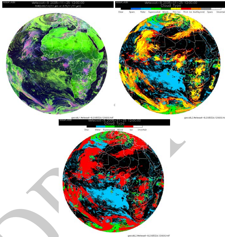
Figure 16: Example results (using SEVIRI) from the ACT algorithm for November 25, 2005. The top, left panel is a RGB false color image and the top, right and bottom, left panels show the cloud type and cloud phase results, respectively.
