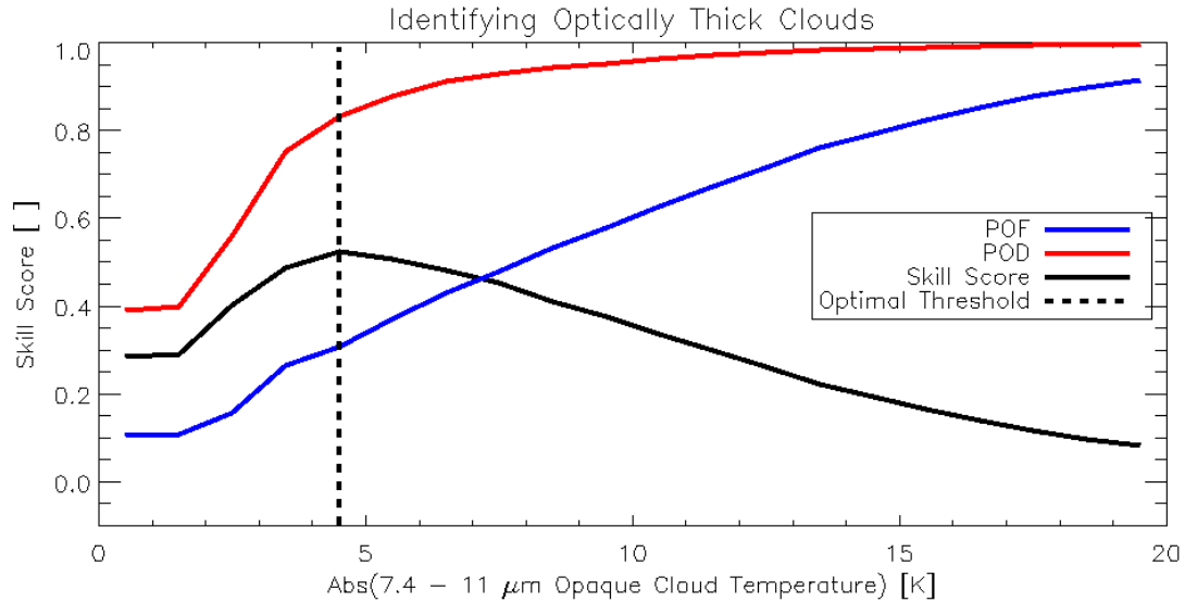
Figure 7: Peirce-Hanssen-Kuipers skill score metrics are shown as a function of the absolute difference in the 7.4 \mu\text{m} – 11 \mu\text{m} opaque cloud temperature ( T_{\text{opaque}}(\text{diff}) ) threshold used to distinguish between clouds with a 11- \mu\text{m} cloud optical depth of less than and greater than 2.0. The probability of false alarm (POF) is shown in blue, the probability of detection (POD) is shown in red, and the skill score is depicted by the black solid line. The T_{\text{opaque}}(\text{diff}) threshold that maximizes the skill score is depicted by the dashed black line. This analysis is based on over 8000 SEVIRI/CALIOP match-ups.
