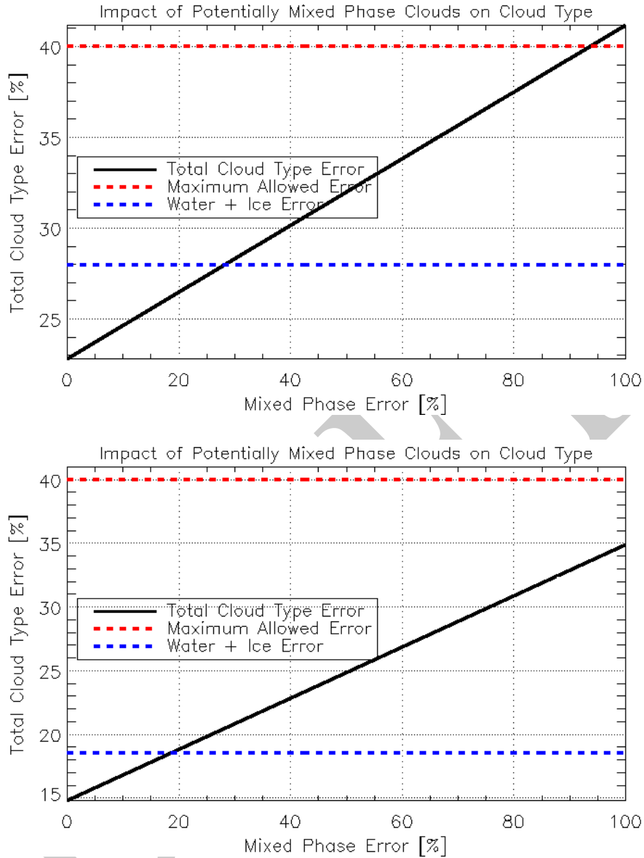
Figure 20: Same as Figure 19, except for cloud type.
