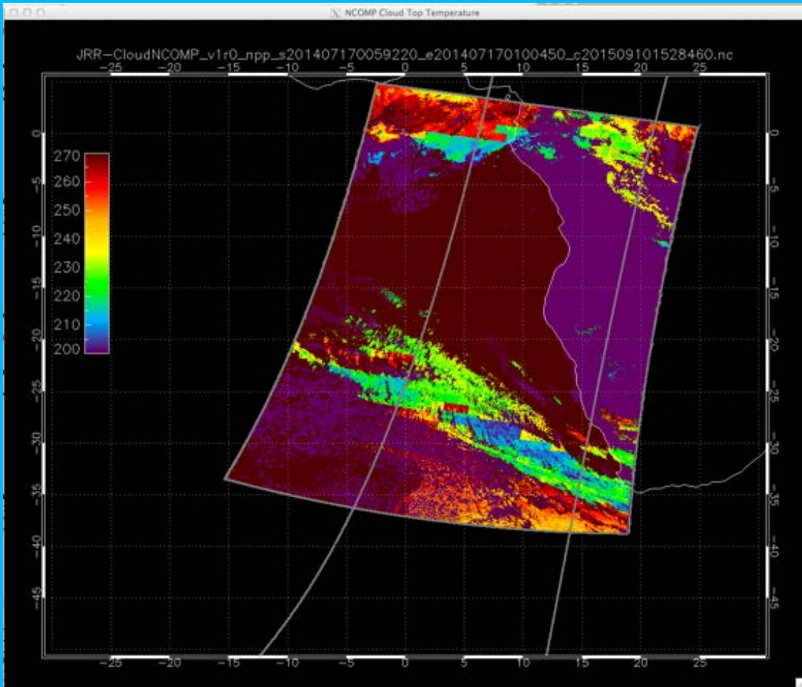
Figure 5. T_{\text{cld}} (K) input from VIIRS Cloud Height/Temperature algorithm for ~0059 UTC, 17 July 2014.
