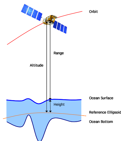
Figure 1 : Altimetric distances – Altitude, Range and Height
