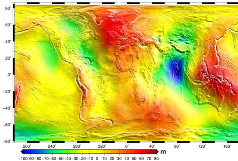
Figure 11 : Mean Sea Surface MSS_CNES-CLS11.
