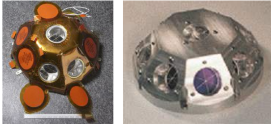
Figure 6 : Jason-3 Laser Reflector Array
