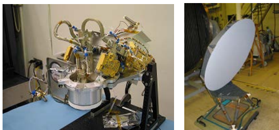
Figure 4 : Jason-3 AMR Instrument and Antenna
