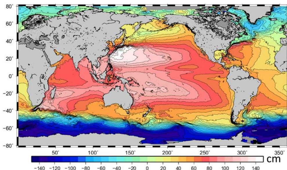
Figure 12 : Mean Dynamic Topography MDT_CNES-CLS09
