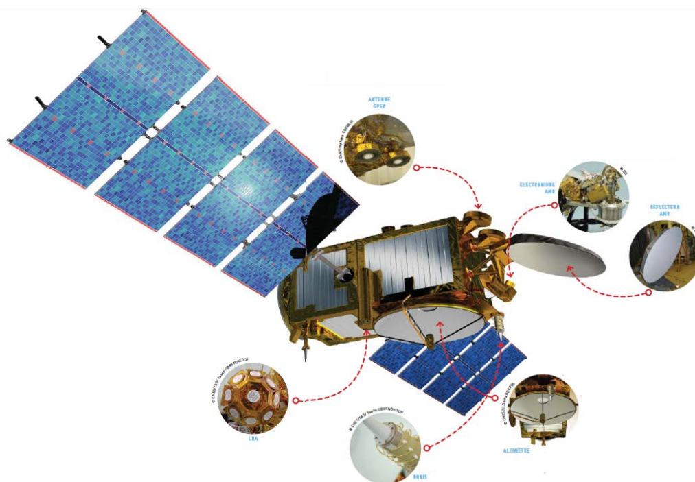
Figure 2 : Main components of the Jason-3 satellite
