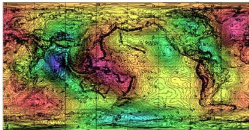
Figure 13 : EGM96 geoid
