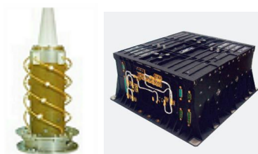
Figure 5 : Jason-3 DORIS Receiver Antenna and Instrument
