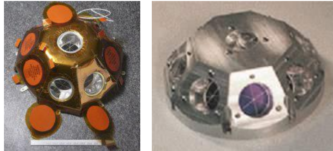
Figure 6 : Jason-3 Laser Reflector Array
