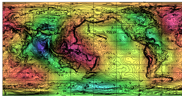
Figure 13 : EGM96 geoid
