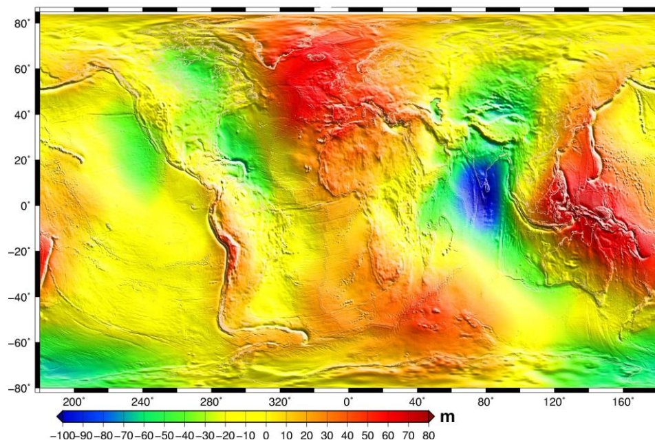
Figure 11 : Mean Sea Surface MSS_CNES-CLS11.
