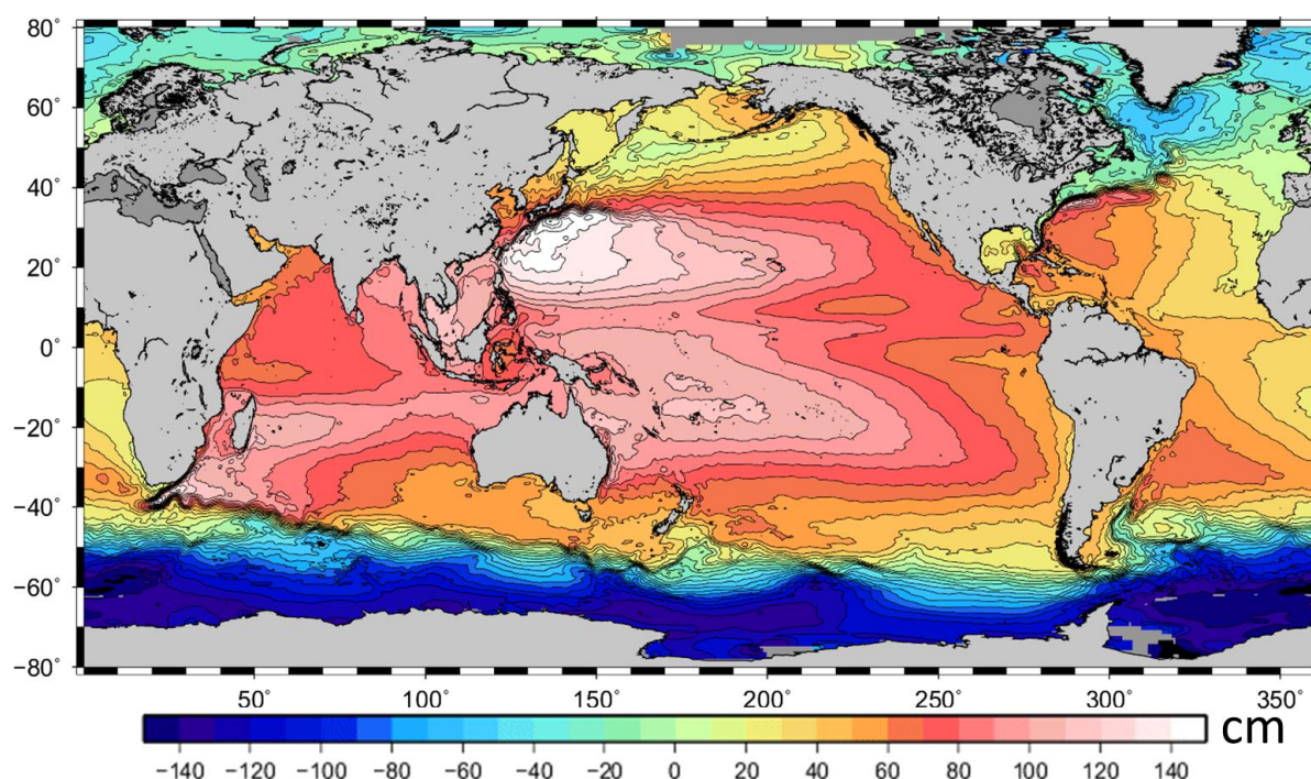
Figure 12 : Mean Dynamic Topography MDT_CNES-CLS09
