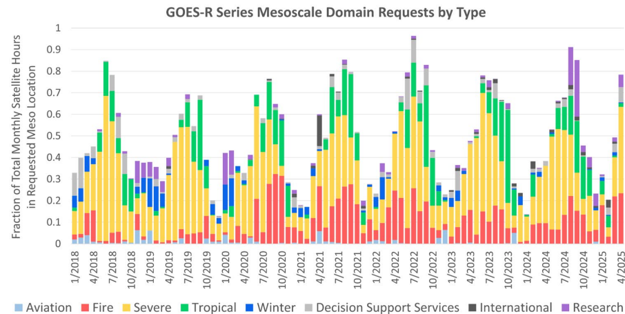
Figure 3. The frequency of mesoscale domain requests varies over time, peaking during summer months.
