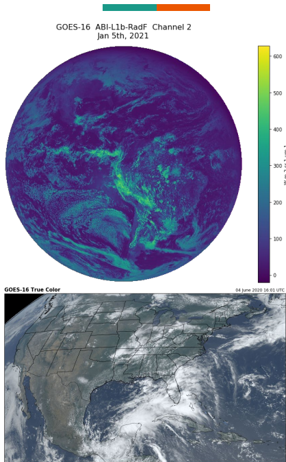
Figure 7. GOES-16 visualized with Python. 7a (top) ABI L1b Channel 2 Full Disk Radiances from Jan 5th, 2021. 7b (bottom): True Color CONUS from June 4th, 2020.
