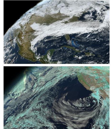
Figure 6. GeoTIFFs created using Geo2Grid. 6a (top): GOES-16 CONUS true color. 6b (bottom): GOES-17 PACUS natural color.
