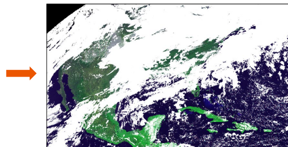
Figure 11. Clear Sky Mask vector layer (left image) is used to mask an RGB-false color raster in QGIS (right image).
